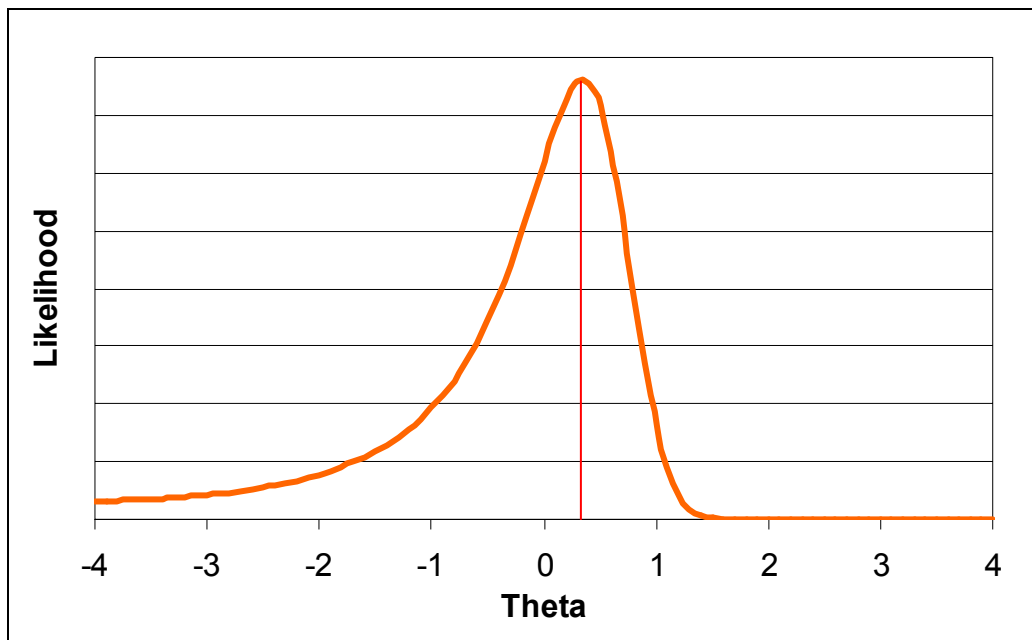
Figure I: A Likelihood Function and Estimated \theta = 0.33
